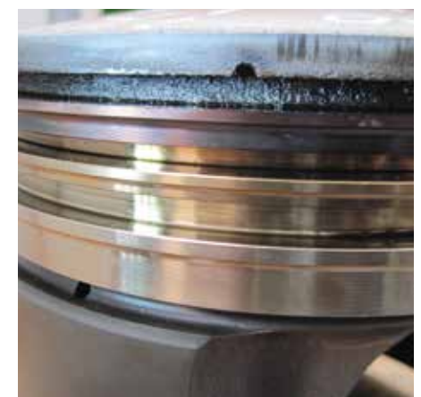
Steel piston with ring grooves INNIO Jenbacher J612 GS-F02
